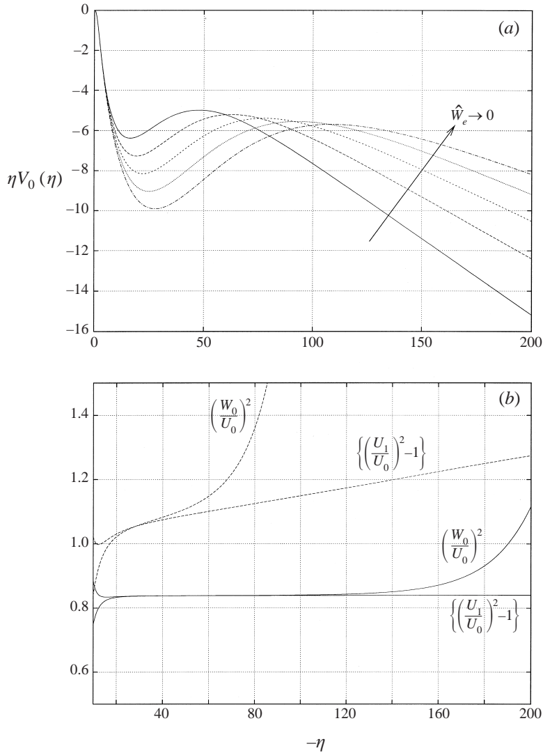
FIGURE 19. (a) The behaviour of \eta V_0(\eta) as \hat{W}_e \rightarrow 0^- . Profiles are shown at \hat{W}_e = 10^{-5}, 10^{-6}, \dots, 10^{-9} . (b) A comparison of (W_0/U_0)^2 and (U_1/U_0)^2 - 1 at \hat{W}_e = 10^{-6} (dashed lines) and \hat{W}_e = 10^{-8} (solid lines).
